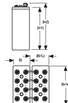
20 OPzV 2500 up to 24 OPzV 3000
