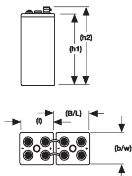
8 OPzV 800 up to 12 OPzV
