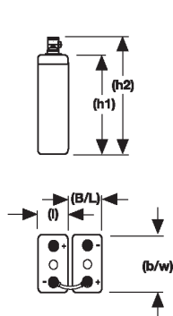
2 OPzV 100 up to 11 OPzV 770
