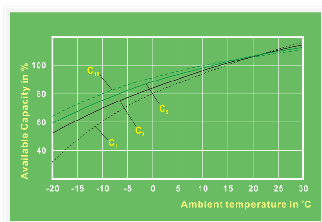
Available capacity in relation to ambient temperature
