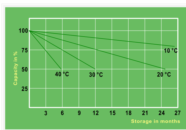
Self-discharge in relation to the storage temperature
